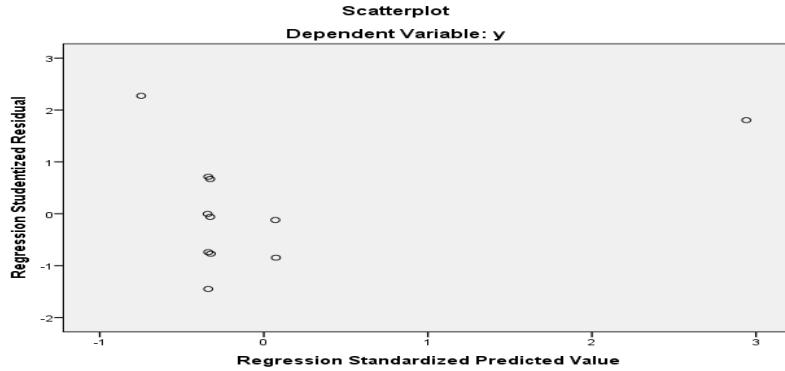
Gambar 4.1 Scatterplot
